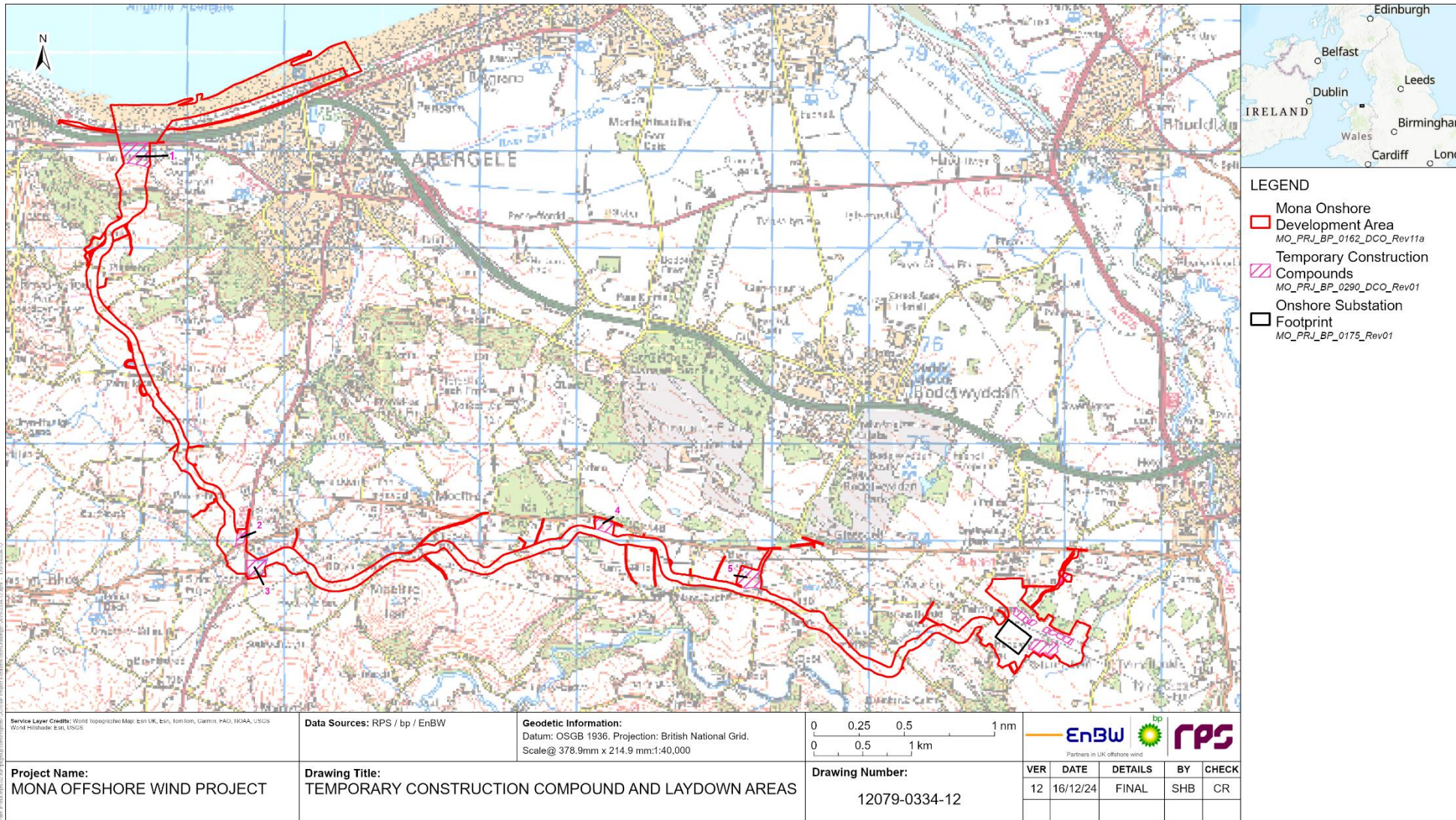
Figure 1.114: Temporary construction compounds and laydown areas.
